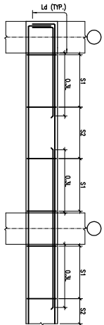
TYP. BEAM R/F DETAILS
