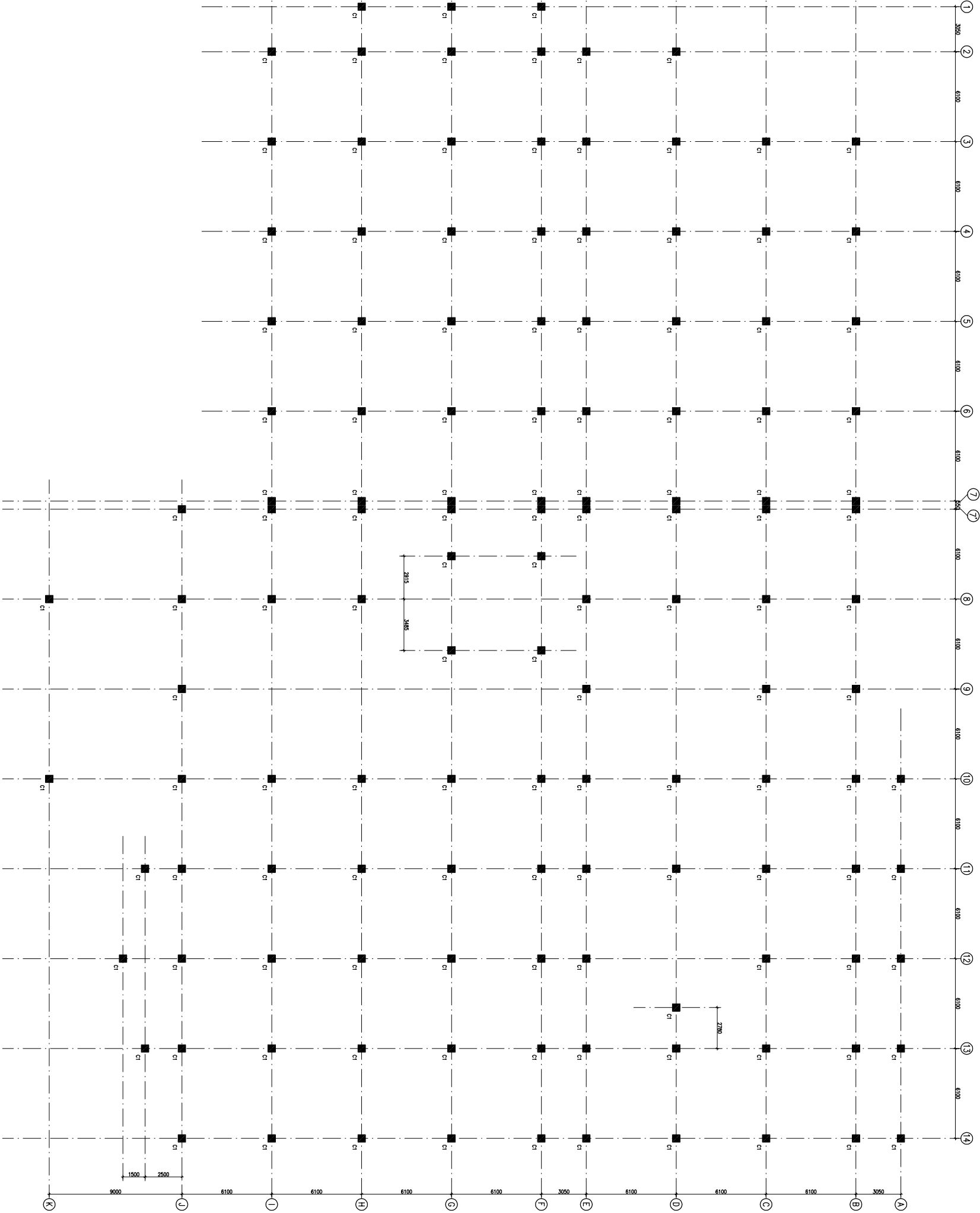
COLUMN LAYOUT PLAN
