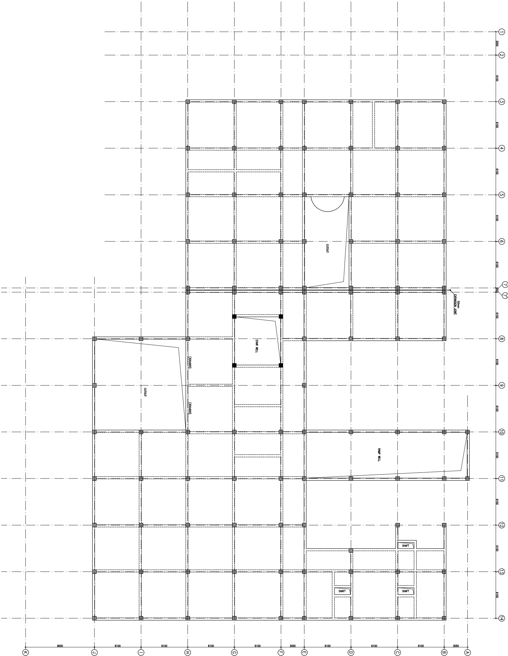
TERRACE LVL. BEAM FRAMING PLAN
