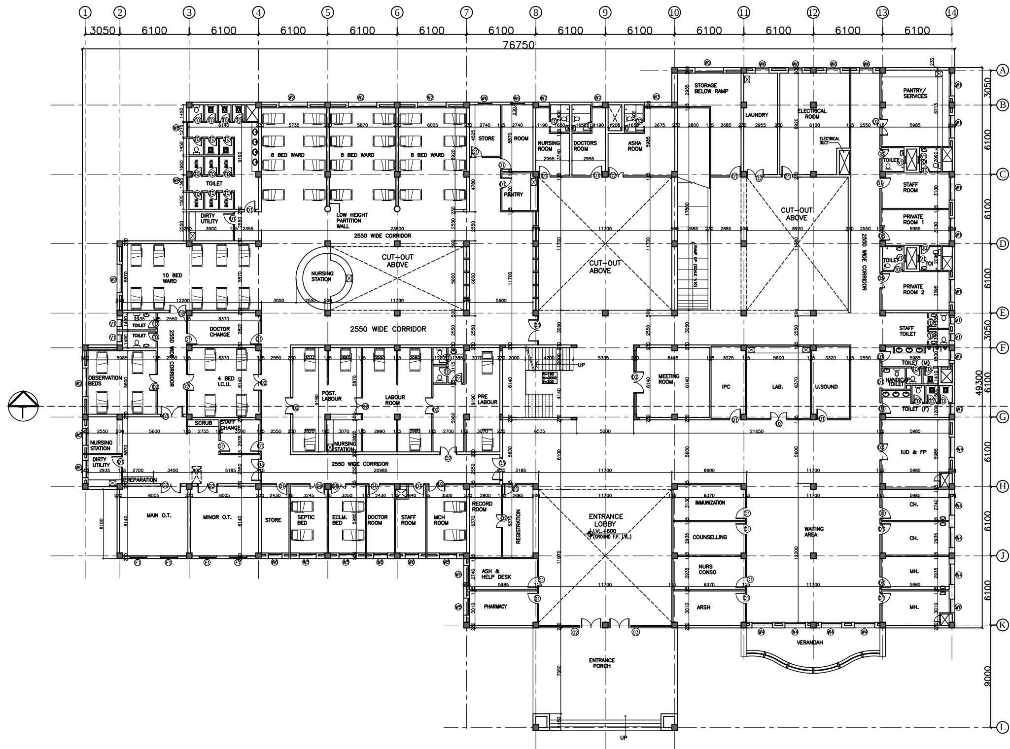
GROUND FLOOR PLAN COVERED AREA – 3022 SQM
