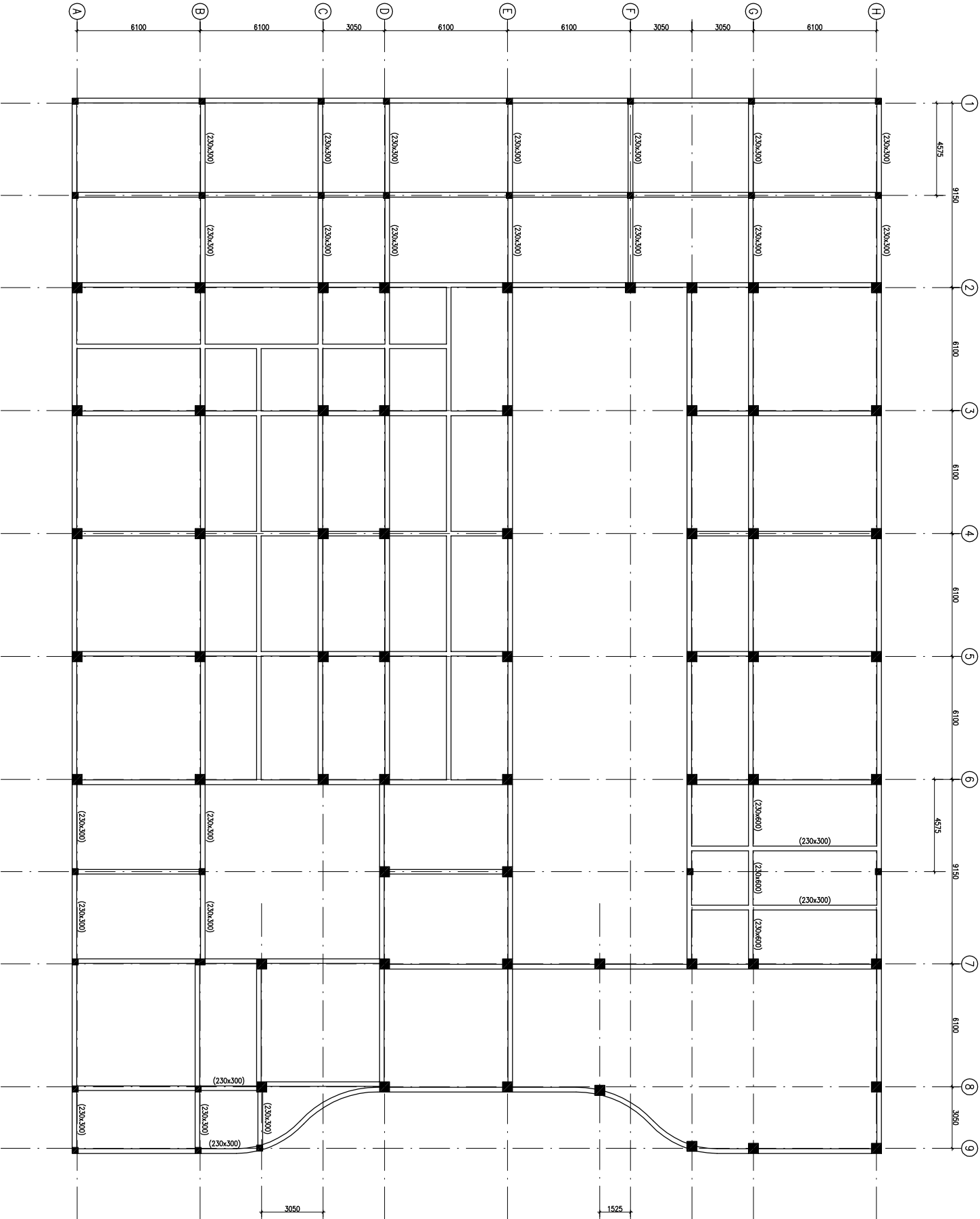
PLINTH BEAM FRAMING PLAN (ALL BEAMS SIZE 230x450 UNO.)
