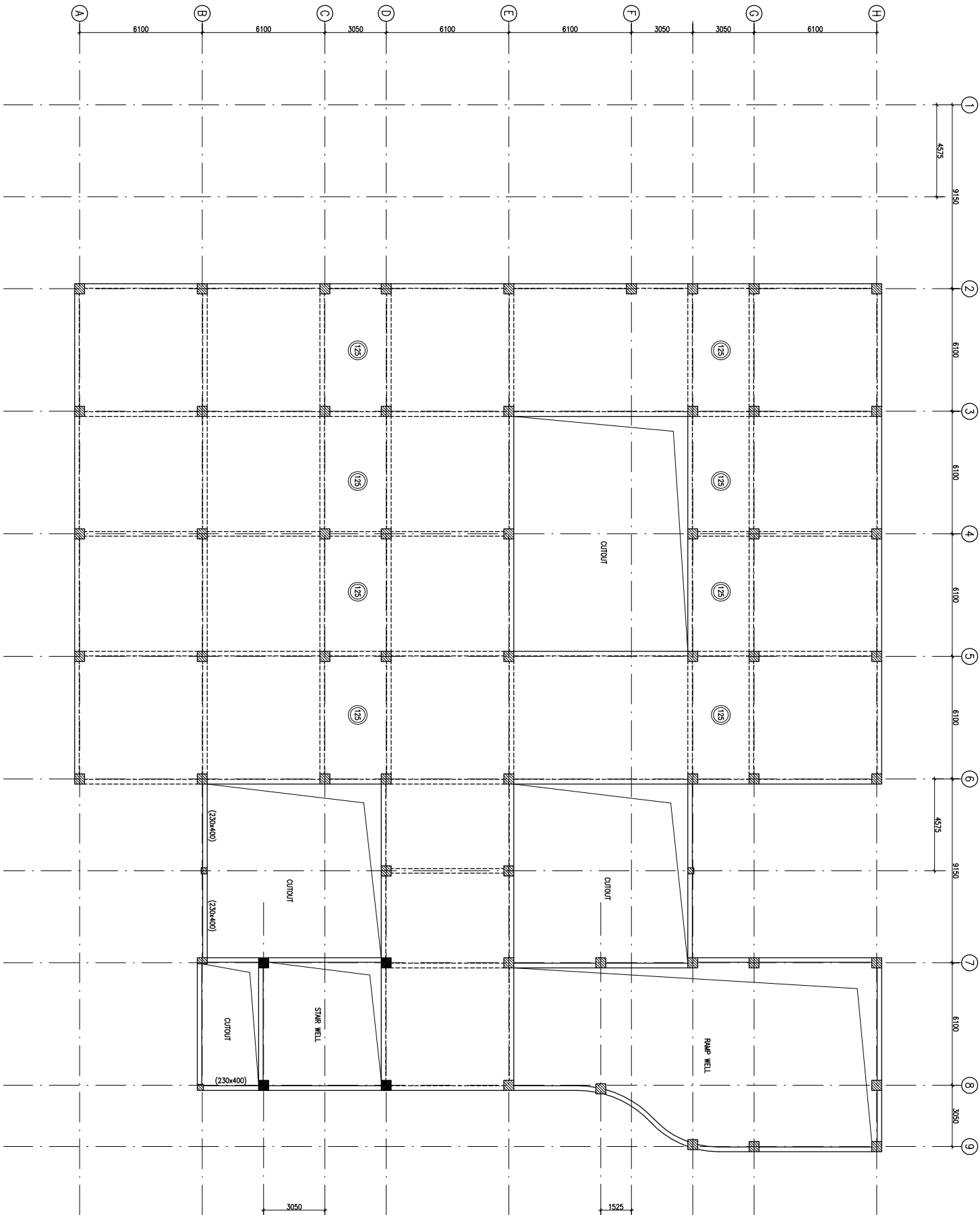
TERRACE LVL BEAM FRAMING PLAN (ALL BEAMS SIZE 230x400 U.N.O.) & (SLAB THICKNESS 150mm U.N.O.)
