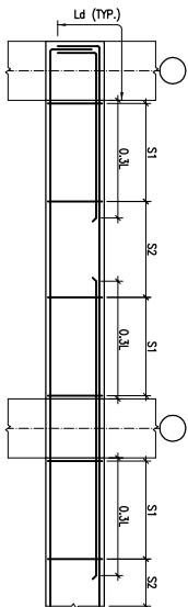
TYP. BEAM R/F DETAILS
