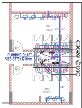
TOILET-01 WATER SUPPLY LAYOUT
