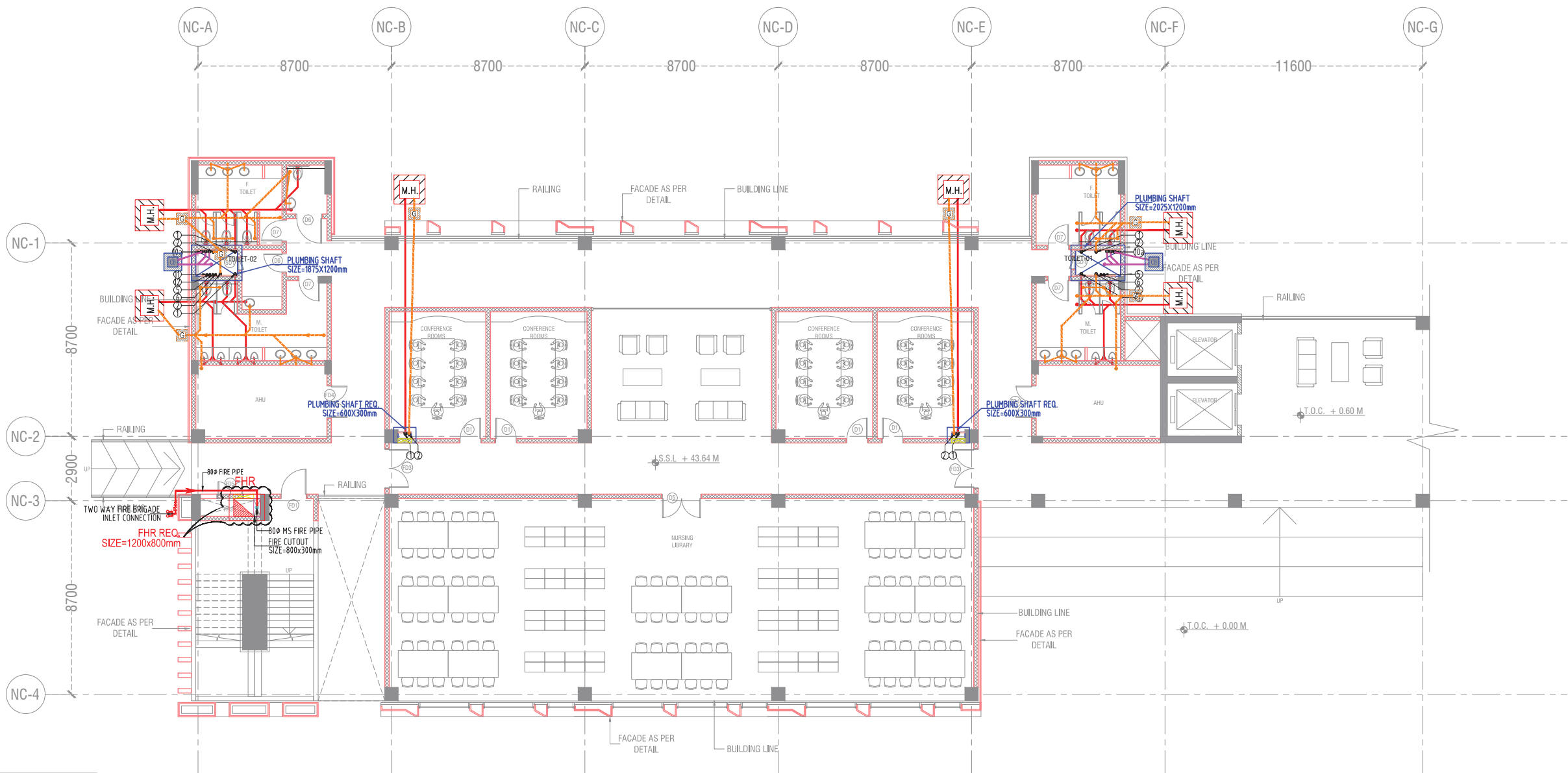
01. GROUND FLOOR PLAN SCALE - 1:100
