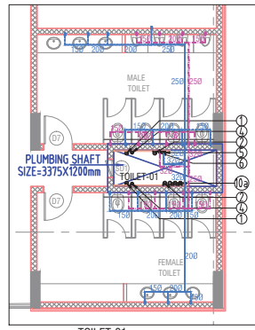
TOILET-01 WATER SUPPLY LAYOUT
