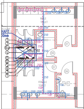
TOILET-02 WATER SUPPLY LAYOUT
