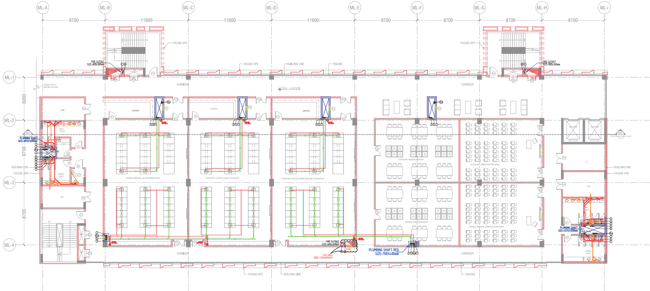
01. SECOND FLOOR PLAN SCALE - 1:125
