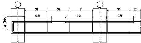
TYP. BEAM R/F DETAILS
