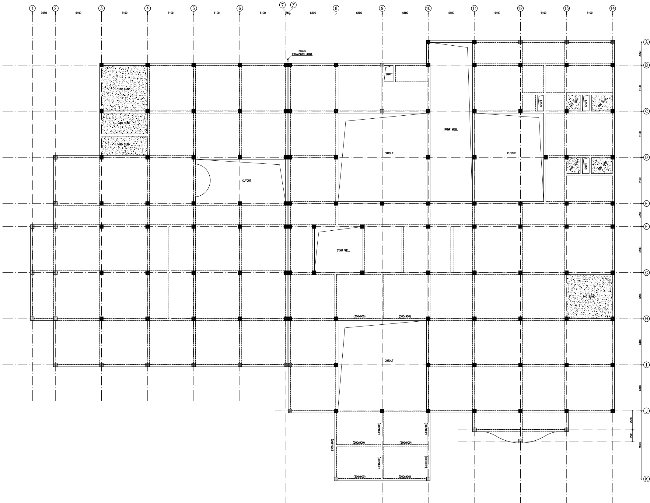
FIRST FLOOR BEAM FRAMING PLAN (ALL BEAMS SIZE 300x900 U.N.G.) & (SLAB THICKNESS 160mm U.N.G.)
