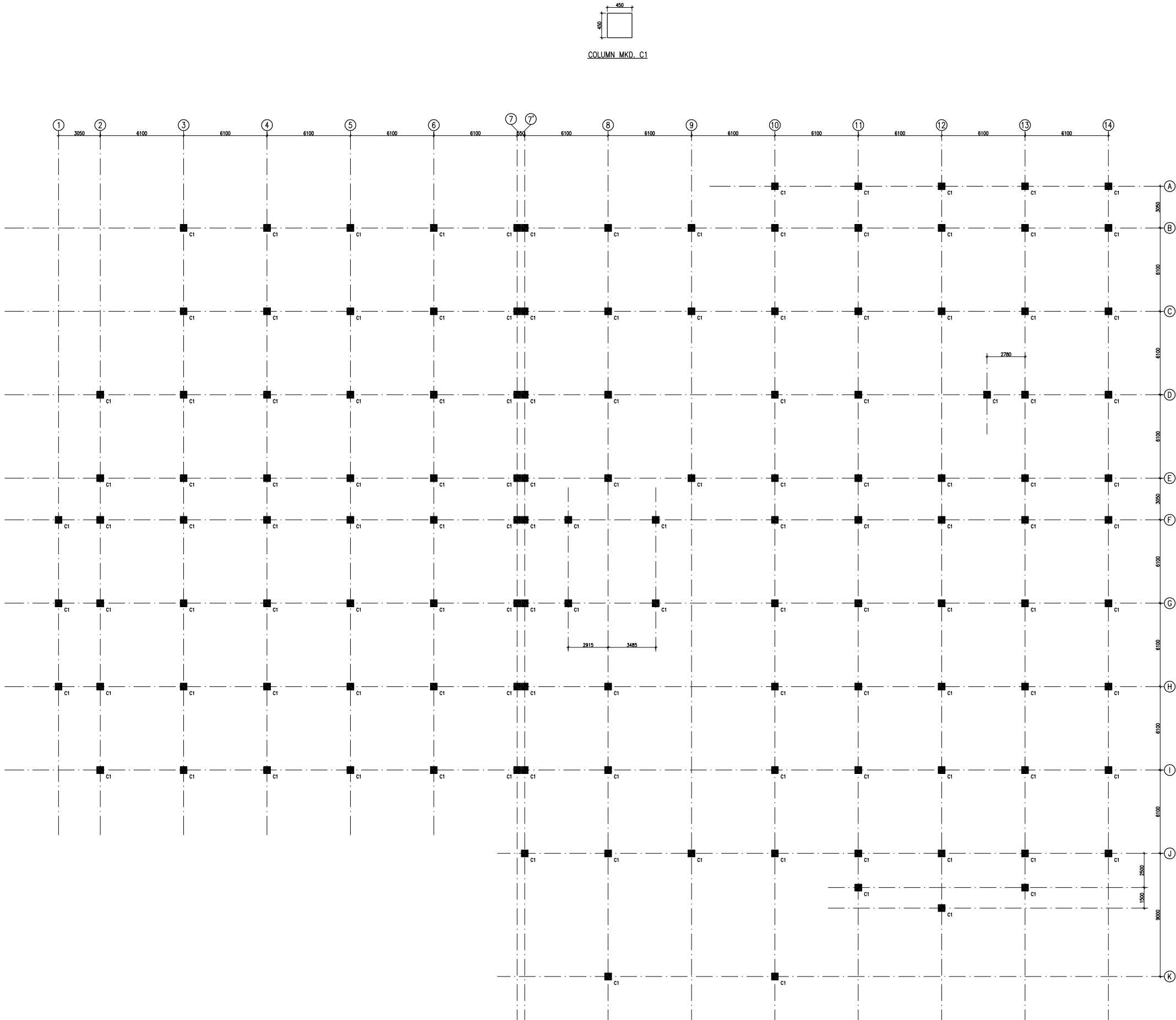
COLUMN LAYOUT PLAN
