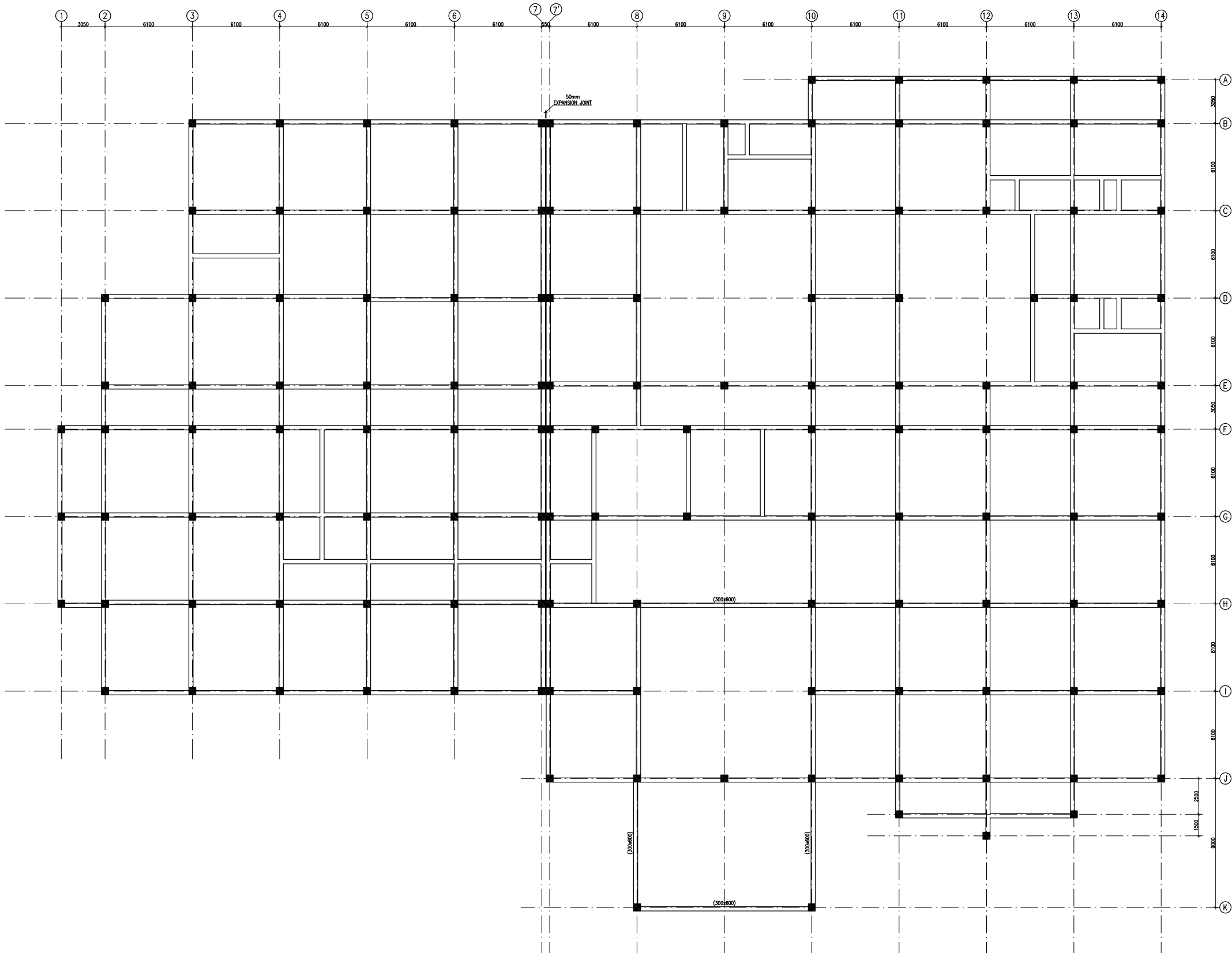
PLINTH BEAM FRAMING PLAN (ALL BEAMS SIZE 300x450 UNLS.)
