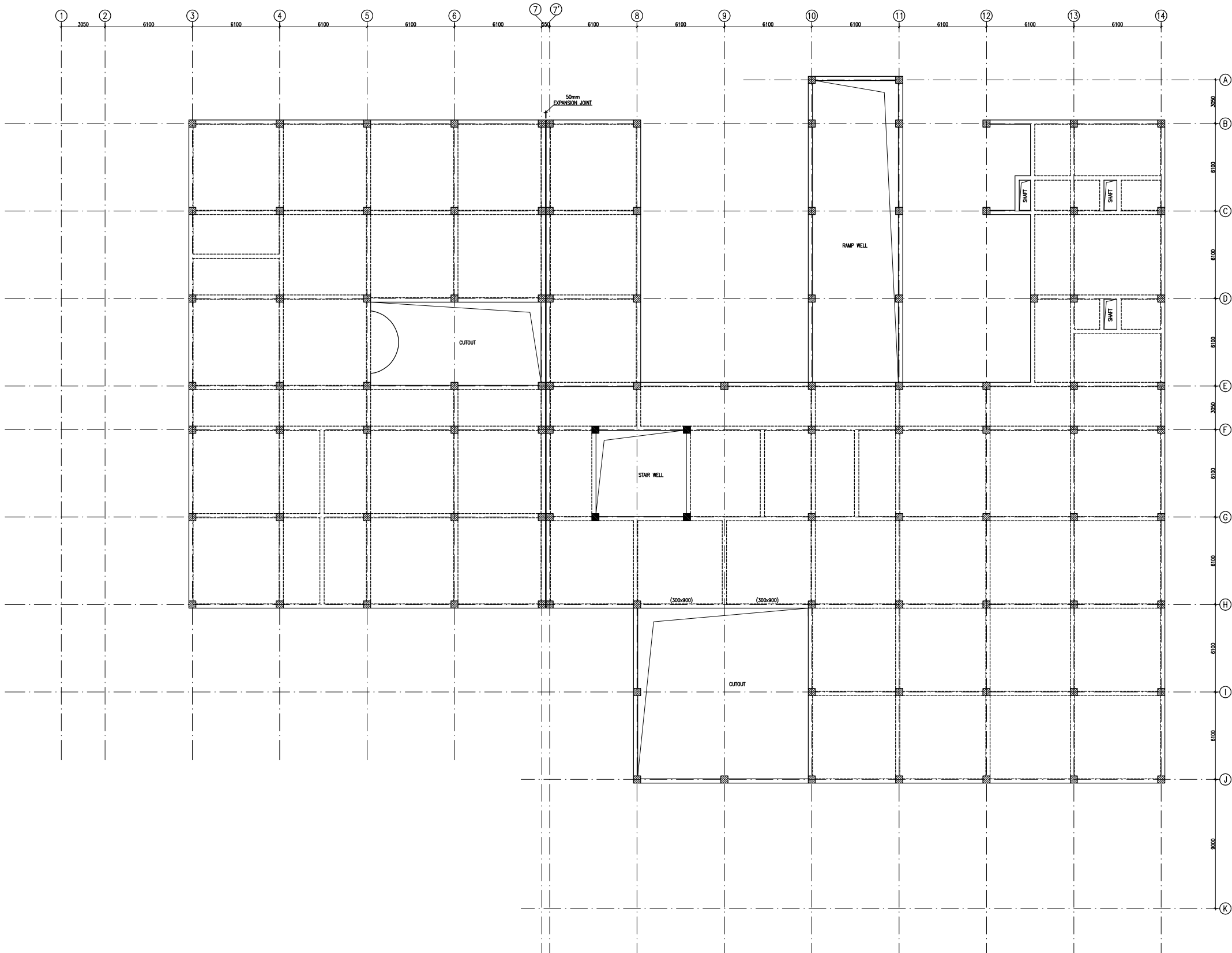
TERRACE LVL. BEAM FRAMING PLAN (ALL BEAMS SIZE 300x600 U.N.O.) & (SLAB THICKNESS 160mm U.N.O.)
