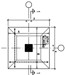
TYPICAL DETAIL OF TAPERED FOOTING
