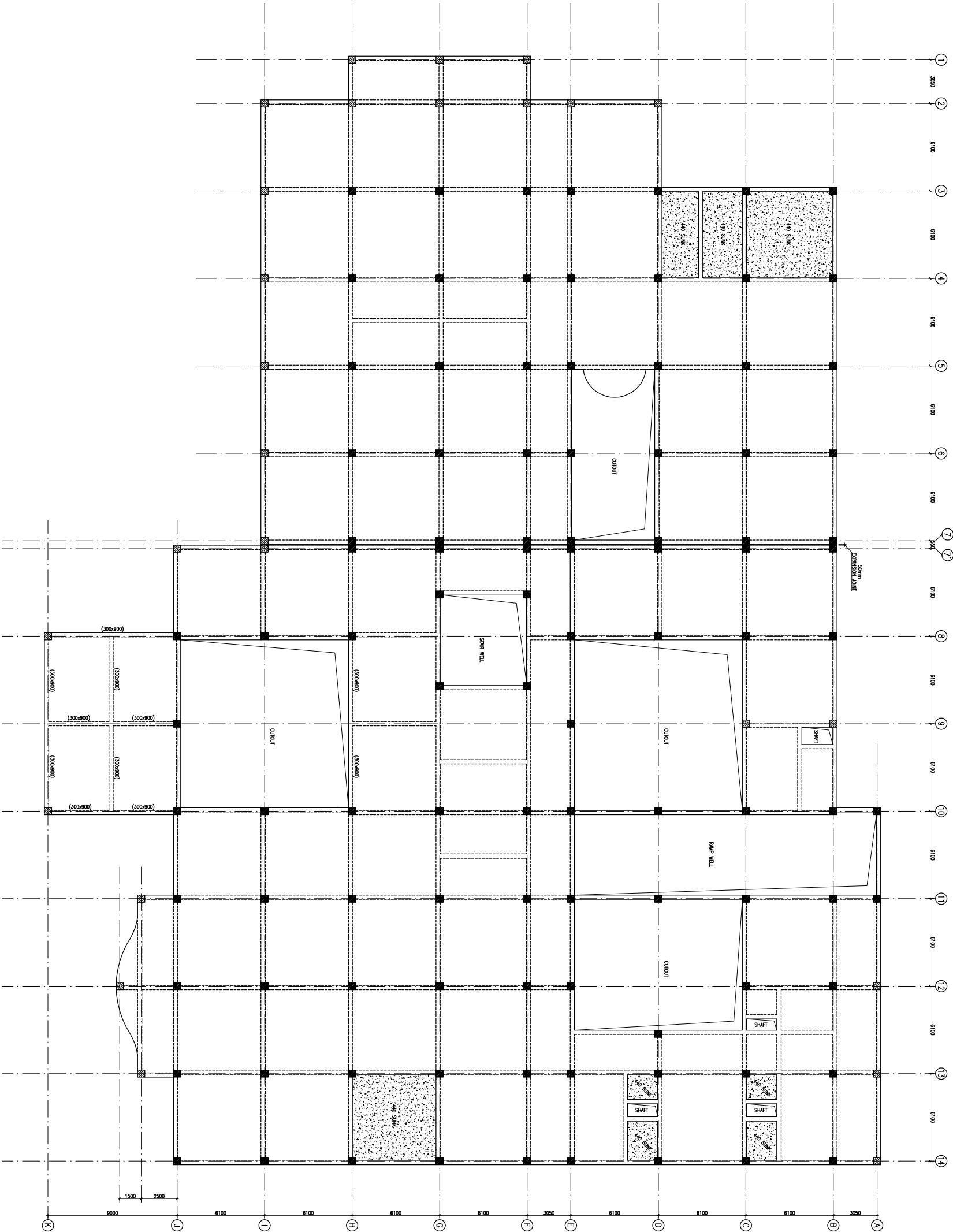
FIRST FLOOR BEAM FRAMING PLAN (ALL BEAMS SIZE 300x900 UNLESS OTHERWISE NOTED)
